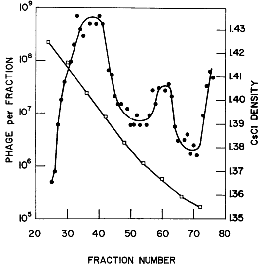
FIG. 4. Equilibrium centrifugation of U3 in CsCl. Density gradient of CsCl ( \square ) and U3 titers per fraction ( \bullet ) are indicated.
