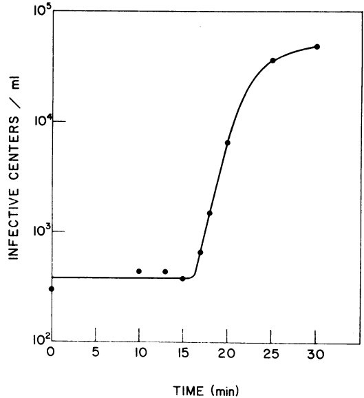
FIG. 1. Single-cycle growth curve.
