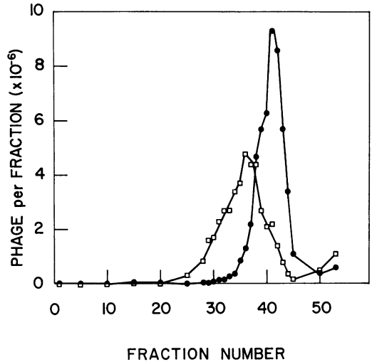
FIG. 5. Sedimentation of U3 and \phi X174 in a sucrose gradient. U3 titers per fraction ( \bullet ) and \phi X174 titers per fraction ( \square ) are indicated. The direction of sedimentation is right to left.
