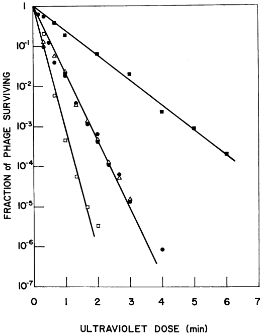
FIG. 3. Ultraviolet inactivation of phages \lambda (■), U3 (●), \phi X174 ( \Delta ), and T4B ( \square ).
