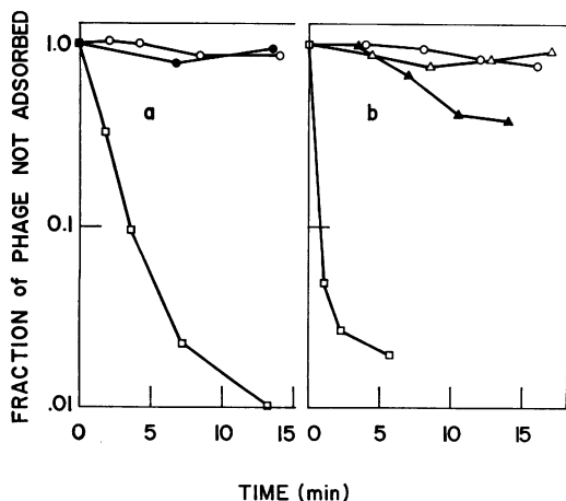
FIG. 2. Adsorption kinetics of phage U3 to cells. (a) U3 + phage adsorbed to strains W3110 (□), SA242 (○), and SA242 grown for several generations in the presence of 5 mM galactose (●). These kinetics are based on cell concentrations of 10^8 per ml. (b) U3 am14 phage adsorbed to strains W3110 (□), SA242 (○), PL2 (△), and PL2 grown for one generation in the presence of 0.02 mM galactose (▲). These kinetics are based on cell concentrations of 2 \times 10^9 per ml.
