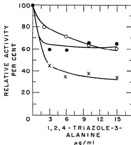
FIG. 8. The effect of 1,2,4-triazolealanine on the formation of several enzymes by E. coli strain W during growth. See Fig. 5 for conditions of growth and for preparation of extracts. The synthesis of Compound III, \bullet — \bullet , was estimated according to the method of Moyed and Magasanik (12); inosinic dehydrogenase, \circ — \circ , was assayed spectrophotometrically (19); and tryptophan synthetase, \times — \times , was estimated by the method of Yanofsky (20).
