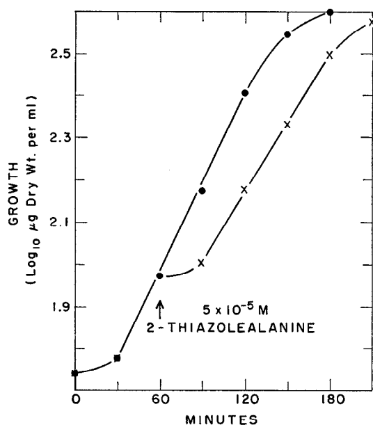
FIG. 4. Transitory inhibition of growth by 2-thiazolealanine. The analogue was added after 60 minutes to one of two parallel cultures of E. coli strain W.
