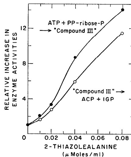
FIG. 5. The effect of 2-thiazolealanine on the formation of enzymes of histidine biosynthesis by E. coli strain W. The cultures were incubated until the cell mass had increased from 30 to 250 µg per ml. Cells from 500 ml of such cultures were centrifuged, washed twice with 0.03 M potassium phosphate buffer at pH 7.4, suspended in 12 ml of buffer, and subjected to sonic oscillation for 5 minutes. The extracts were clarified by centrifugation at 18,000 \times g for 15 minutes. Protein was determined by the Biuret method with crystalline bovine serum albumin as the standard. The synthesis of Compound III and its conversion to ACP and IGP were estimated according to the method of Moyed and Magasanik (12). One mg of protein in the extract prepared from cells grown in the absence of 2-thiazolealanine synthesized 0.053 µmole of Compound III per hour and converted 0.042 µmole of Compound III to ACP per hour. Compound III synthesis was measured in the absence of an amino donor which prevented its conversion to ACP. The conversion of Compound III to ACP was estimated in the absence of ATP and 5-phosphoribosyl-1-pyrophosphate, the substrates for Compound III synthesis.
